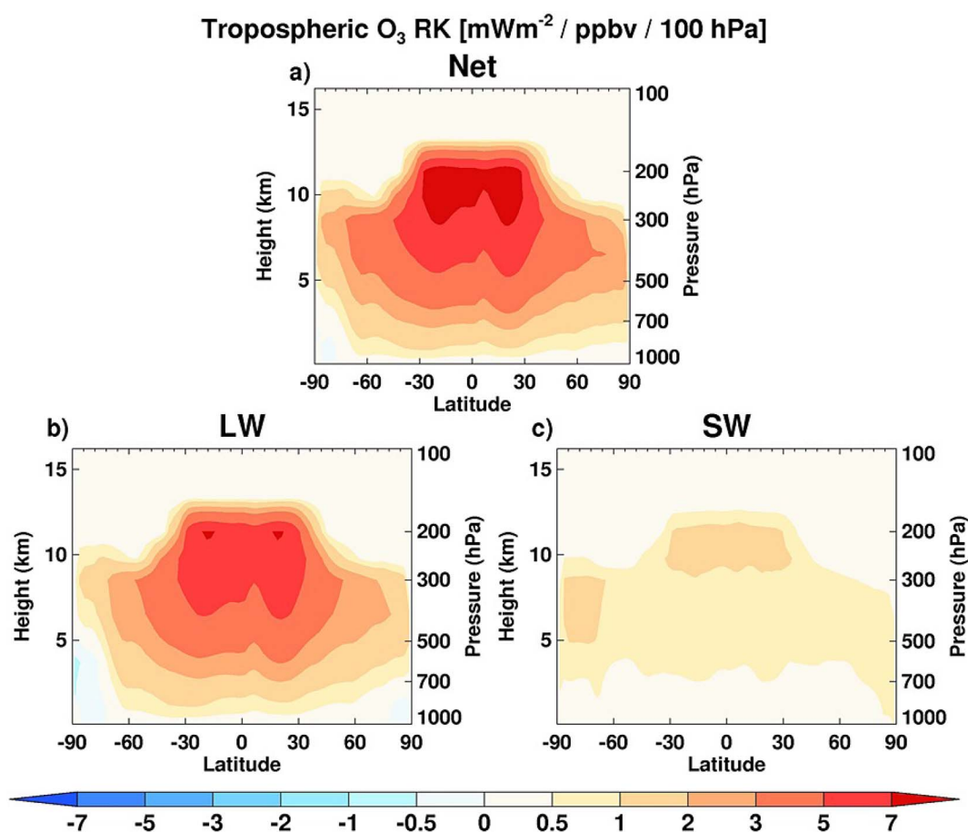
Fig. 11 Annual zonal mean tropospheric ozone radiative kernel (RK) 75 under all-sky conditions in units of \text{mW m}^{-2} \text{ppbv}^{-1}/100 \text{ hPa} for (a) net (LW + SW), (b) LW, and (c) SW. SW (short-wave) refers to the RF resulting from changes in the absorbed solar-radiation by the Earth-atmosphere system, which is mostly incident in the wavelength range 0.2 to 4 \mu\text{m} . LW (longwave) refers to changes in the outgoing longwave radiation at the top of the atmosphere; LW radiation (mostly in the wavelength range 4 to 400 \mu\text{m} sometimes) originates from emission by the Earth and its atmosphere and is modulated by absorption by atmospheric constituents. Radiative forcing is the sum of the individual SW and LW RFs. Note that this illustrates the general radiative response from tropospheric ozone, formed from precursor emissions of \text{NO}_x , CO, \text{CH}_4 , HCs and is not an aviation perturbation. From Rap et al. (2015). 70
